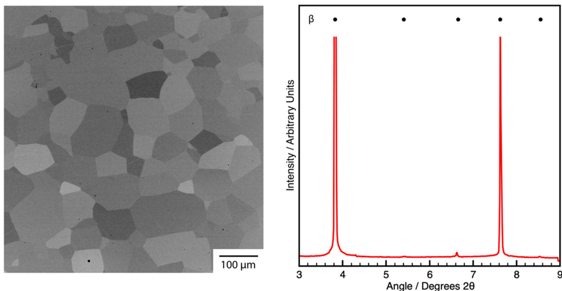
Figure 1. The initial microstructural condition of the alloy, showing recrystallised \beta grains and the sXRD pattern confirming the sample is single phase \beta .
