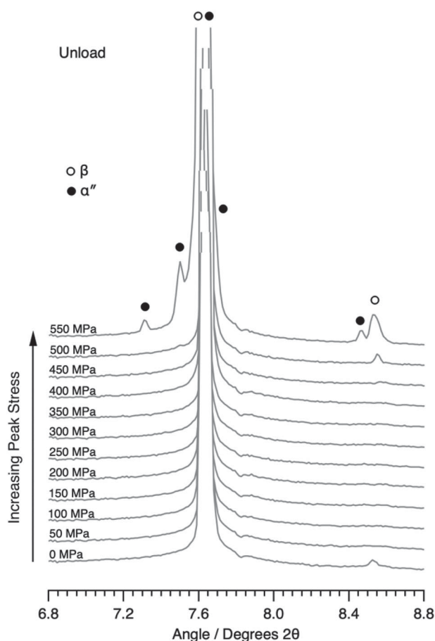
Figure 3. The sXRD diffraction patterns at unload, following each cycle in the incremental stress test. Retained \alpha'' is seen in the microstructure following the cycle to 550 MPa.
